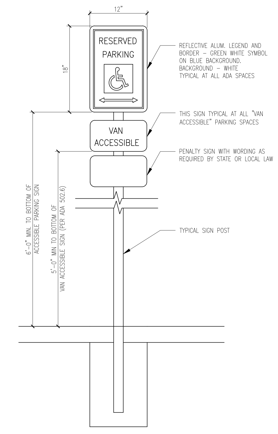
2 HANDICAP PARKING SIGN SCALE: 1"=1'-0"
